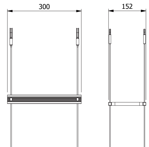
WIRE LADDER COMPARISON: WIDE WIRE LADDER & WIRE LADDER
