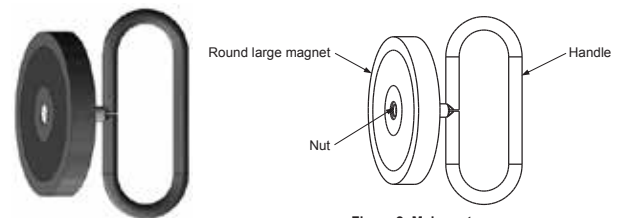
Figure 2: Main parts
